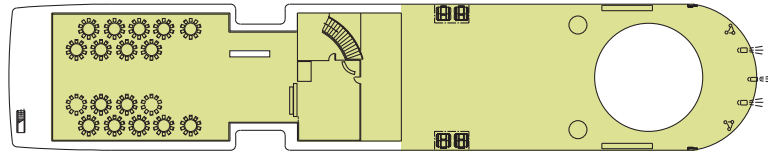
pinnacle deck
